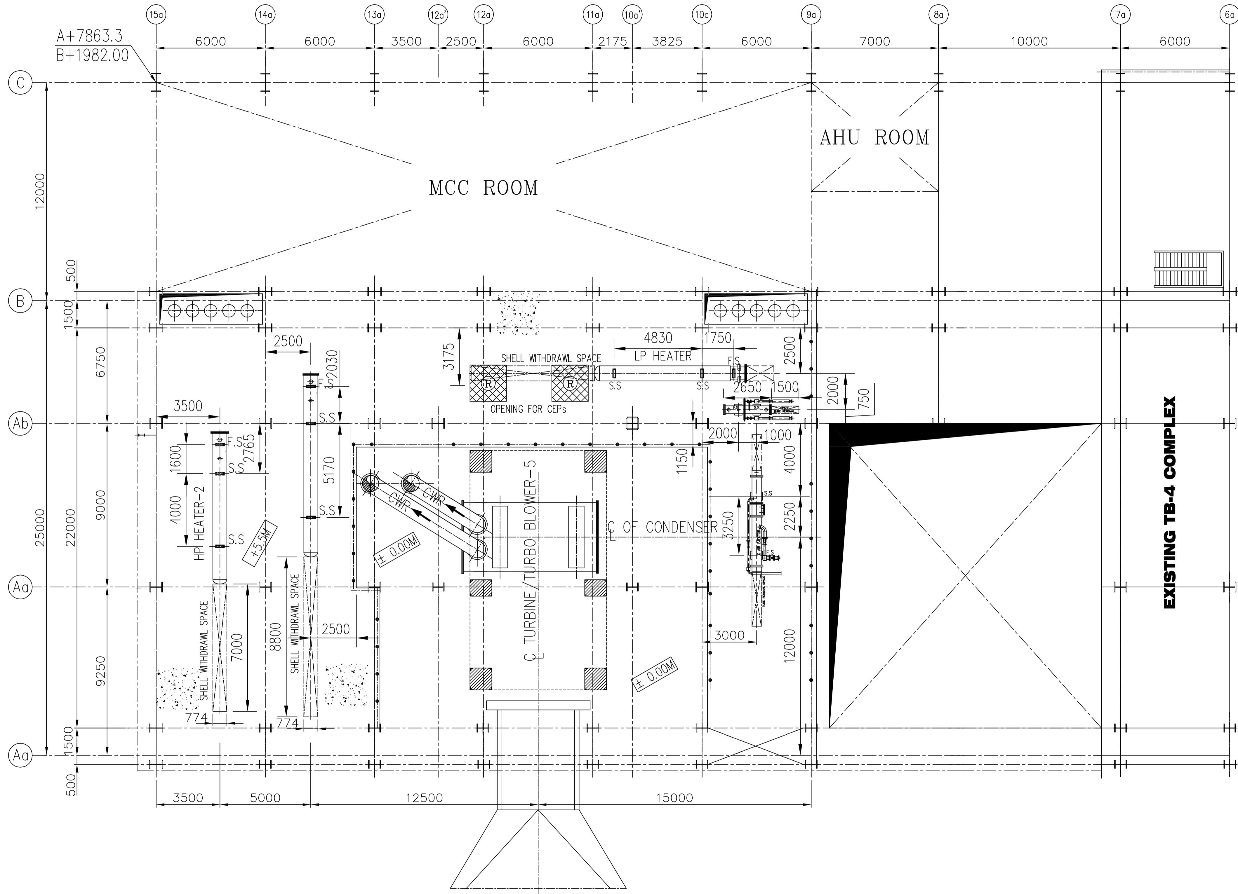
PLAN AT EL. 5.5M
