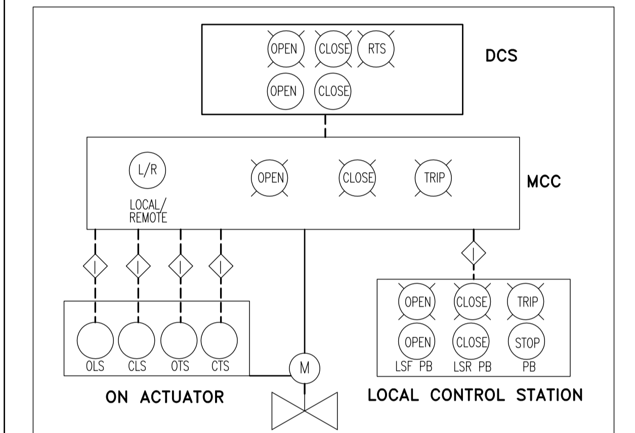
TYPICAL ARRANGEMENT FOR MOTOR OPERATED VALVES ON/OFF (NON INTEGRAL) TYPE
