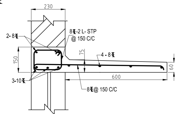
DETAILS OF LINTEL CUM SUNSHADE
