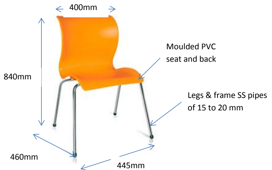
Fig.4 Typical stackable Chair details
