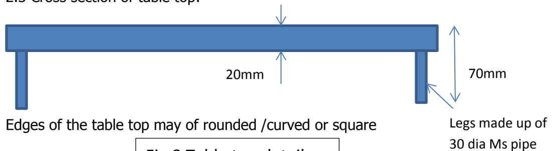
Fig.3 Table top details
