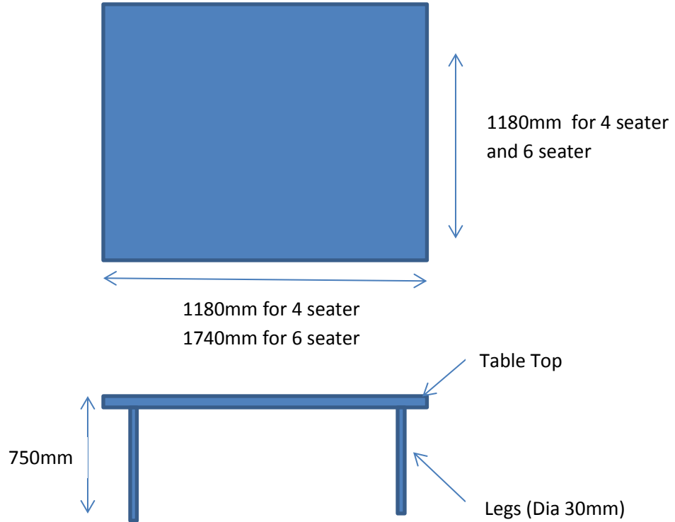
Fig.2 Typical Dimensions Dining table (1+4)
