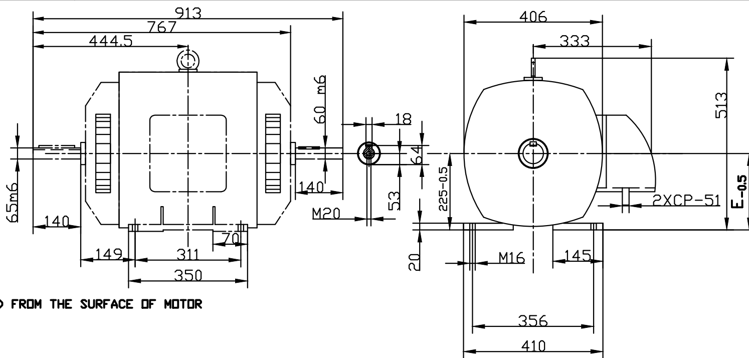
OVERALL DIMENSIONS
