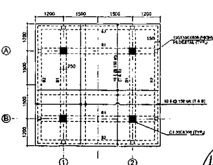
RCC FLOOR DETAILS AT EL. (+)5.40 M (TOC) SLAB THICKNESS = 150 MM
