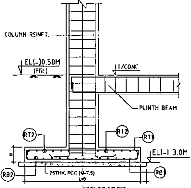
SECTION 1-1
