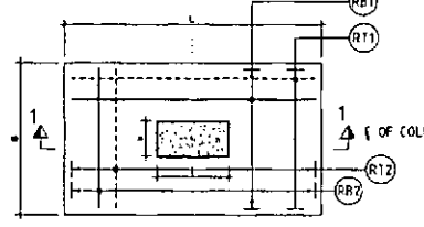
TYPICAL FOOTING REINFT. PLAN
