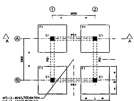
FOUNDATION & PLINTH BEAM LAYOUT PLAN
