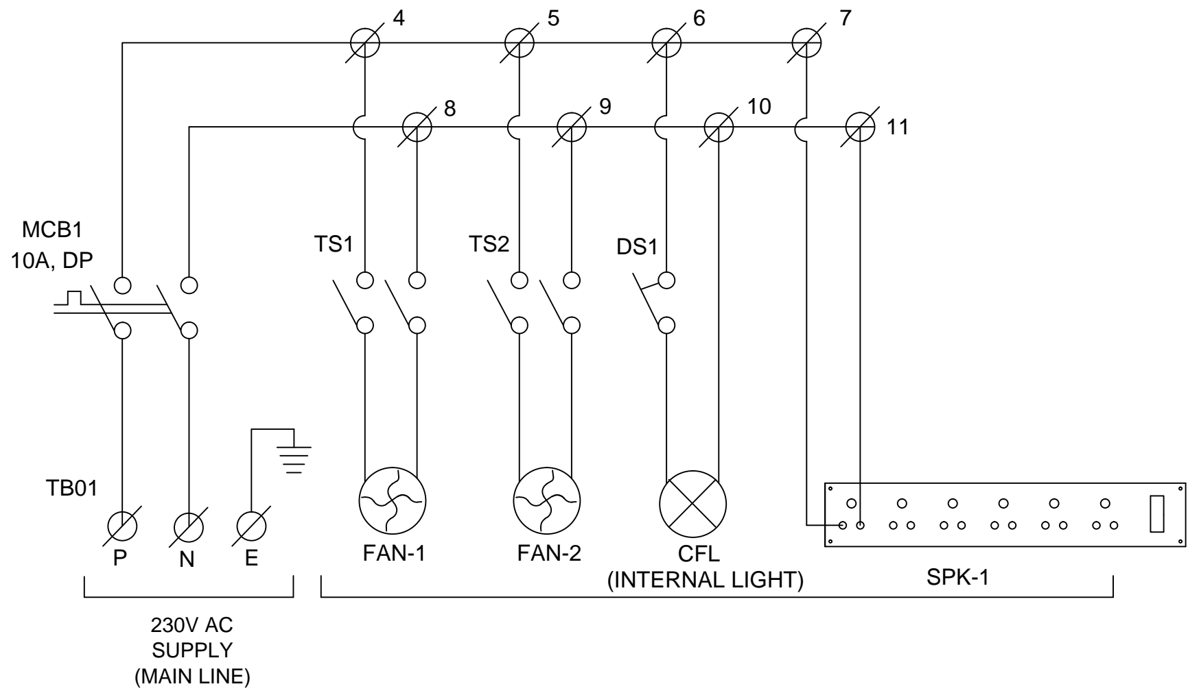
WIRING DRG. FOR EACH SECTION
