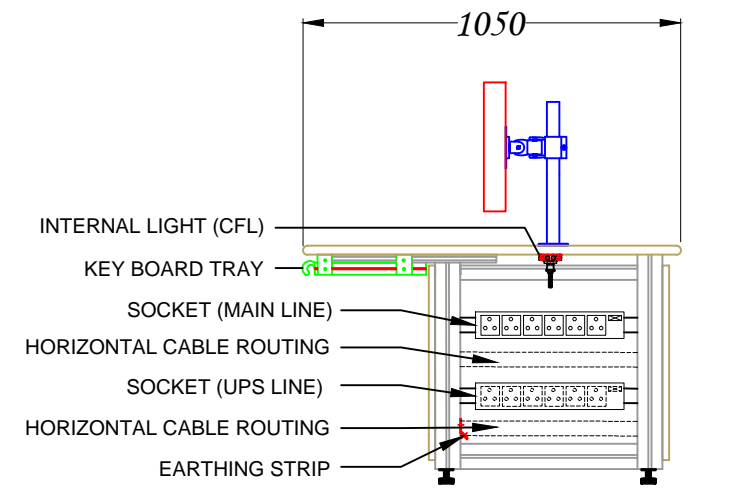
SECTIONAL SIDE VIEW
