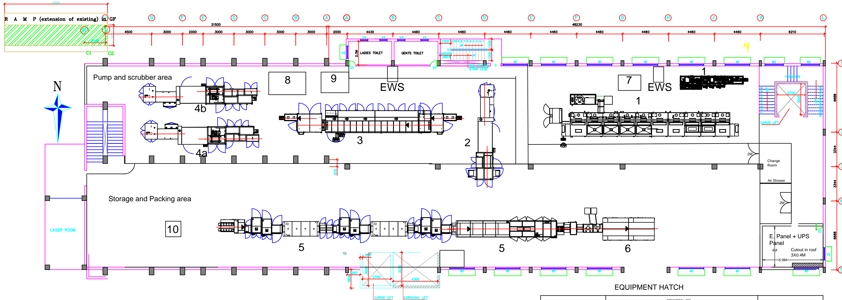
PLAN AT FIRST FLOOR LEVEL
