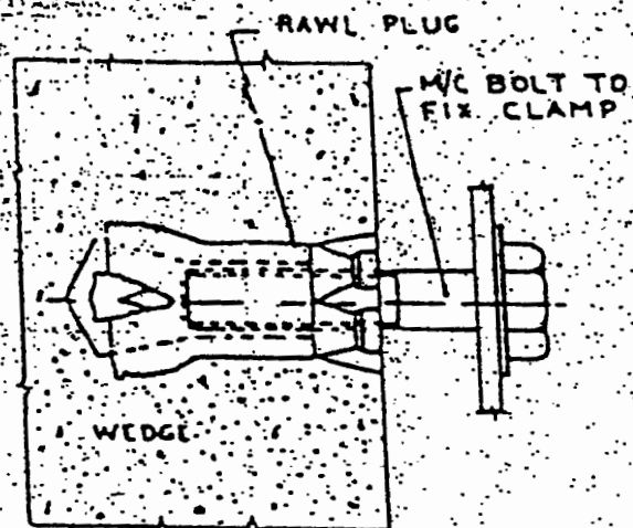
DETAIL - A
