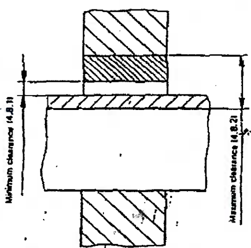
Figure 4 - Clearance fit
