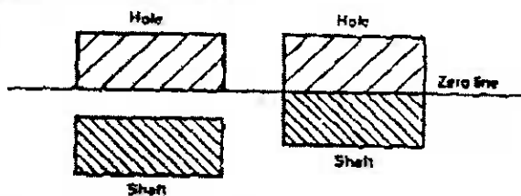
Figure 8 - Schematic representation of clearance fit
