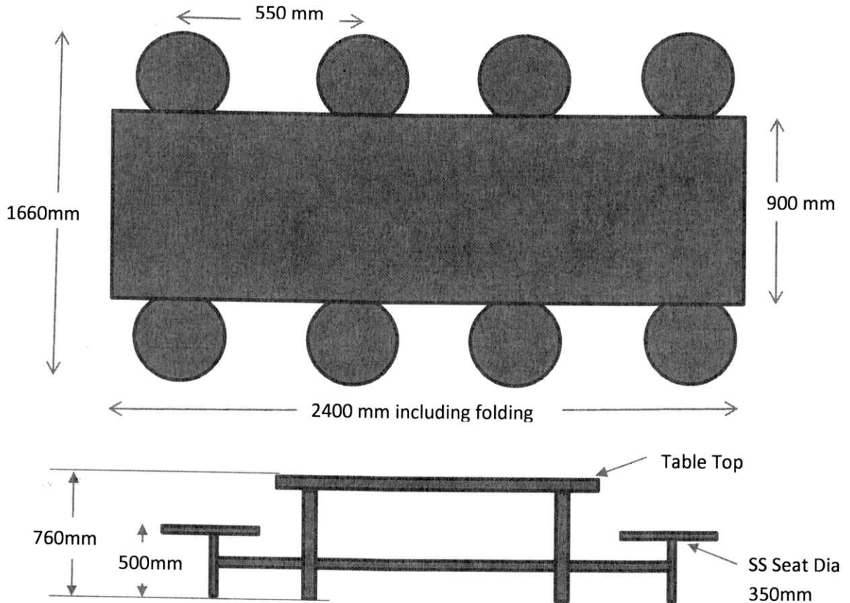
Fig.2 Typical Dimensions Dining table (8 seats)
