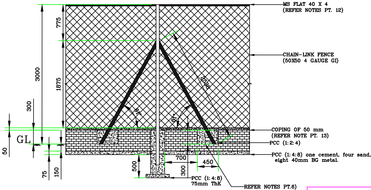
SECTIONAL ELEVATION WITH ISA 50X50X6 STRUT POSTS (REFER NOTES PT. 6)
