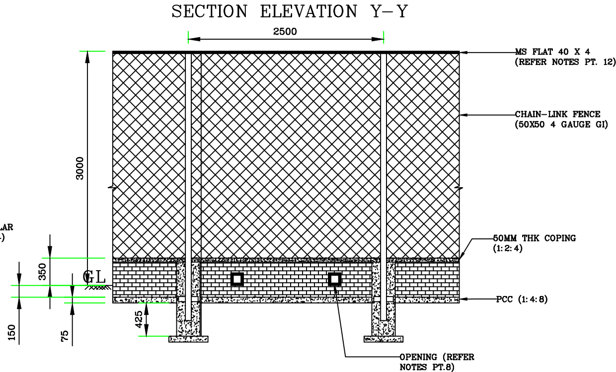
SECTIONAL ELEVATION Y-Y
