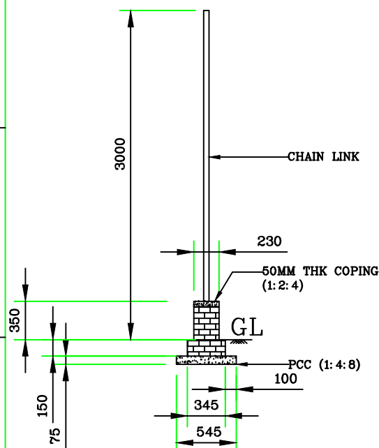
SECTION AT TOE-WALL
