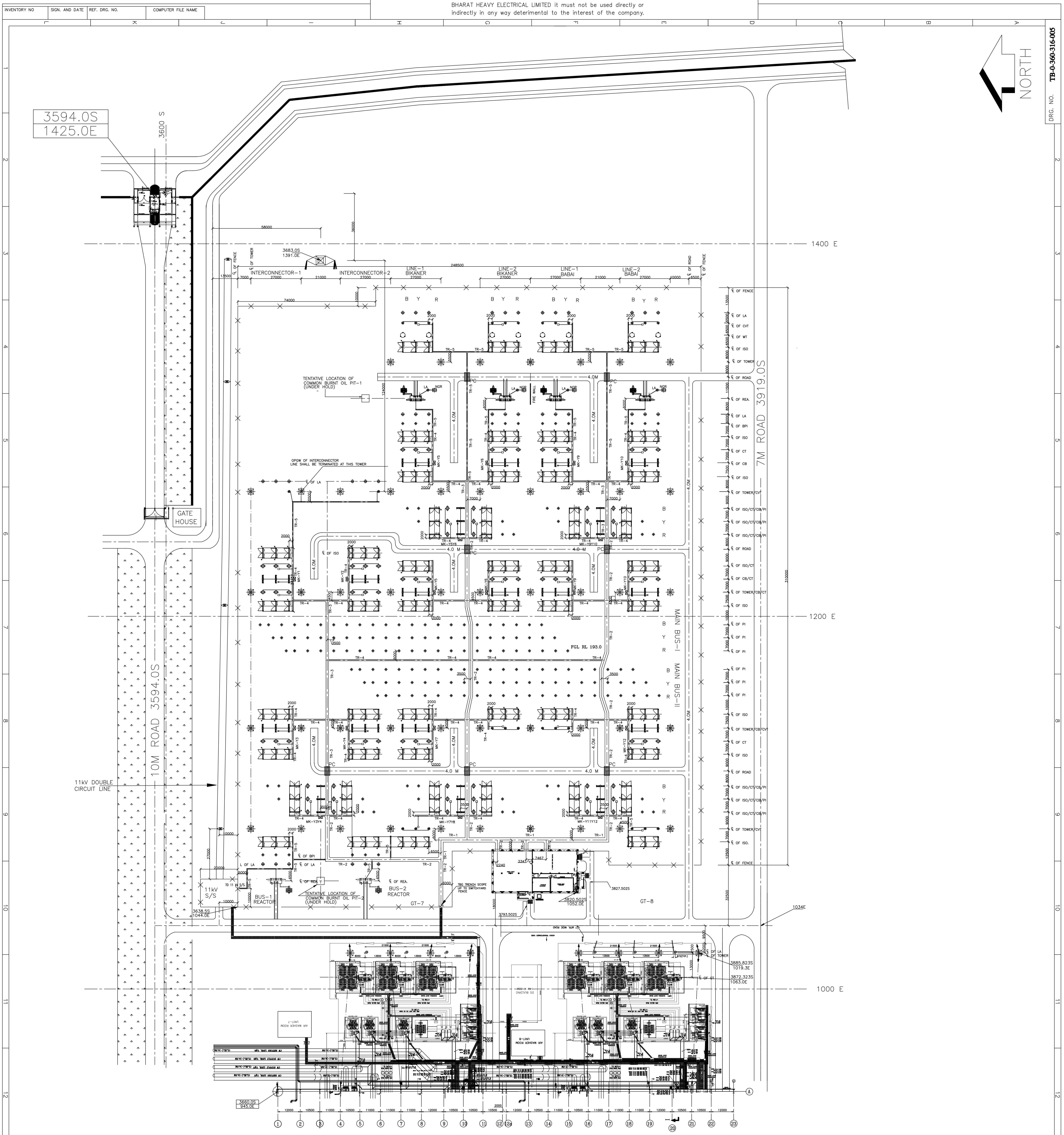
TRENCH LAYOUT PLAN OF UNIT-7 & 8 420kV SWITCHYARD
