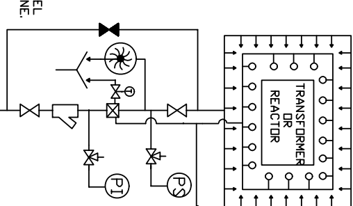
TYPICAL ARRANGEMENT OF HVV SPRAY SYSTEM
