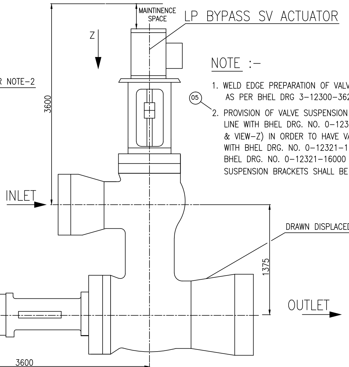
SCHEMATIC ARRANGEMENT OF ANGLE TYPE VALVE
