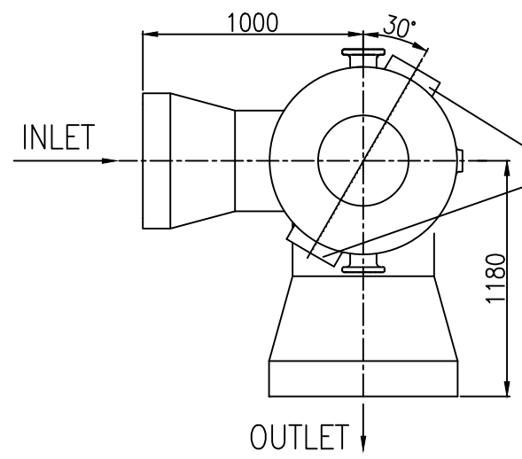
VIEW-Z (WITHOUT ACTUATOR)
