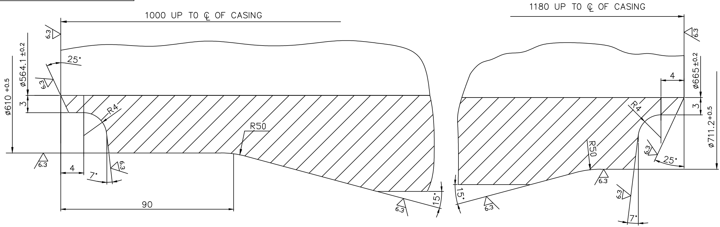
02 EDGE PREPARATION DETAIL AFTER HYDRAULIC TESTING (STEAM INLET SIDE) (PRELIMINARY)
