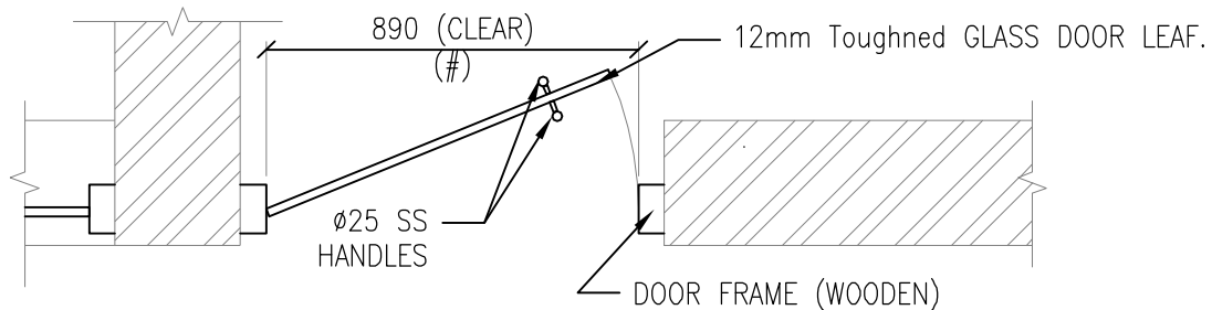
PLAN SCALE 1:20
