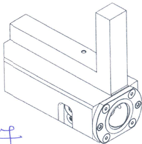
Figure-2.0 (Special Holder)
