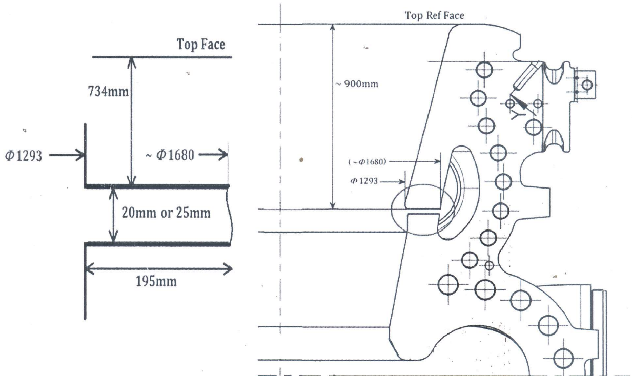
Figure-1 (Drawing of IP Inner Casing - Deep Groove)
