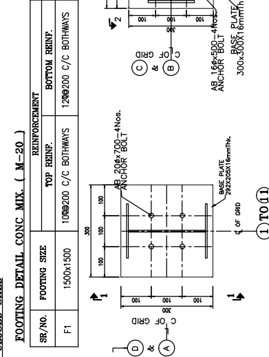
DETAIL I-I
