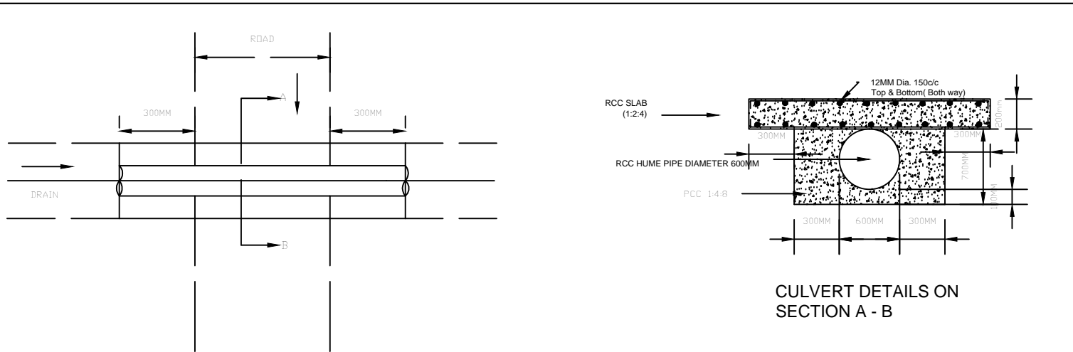
CULVERT DETAILS FOR 600MM DIA,RCC HUME PIPE
