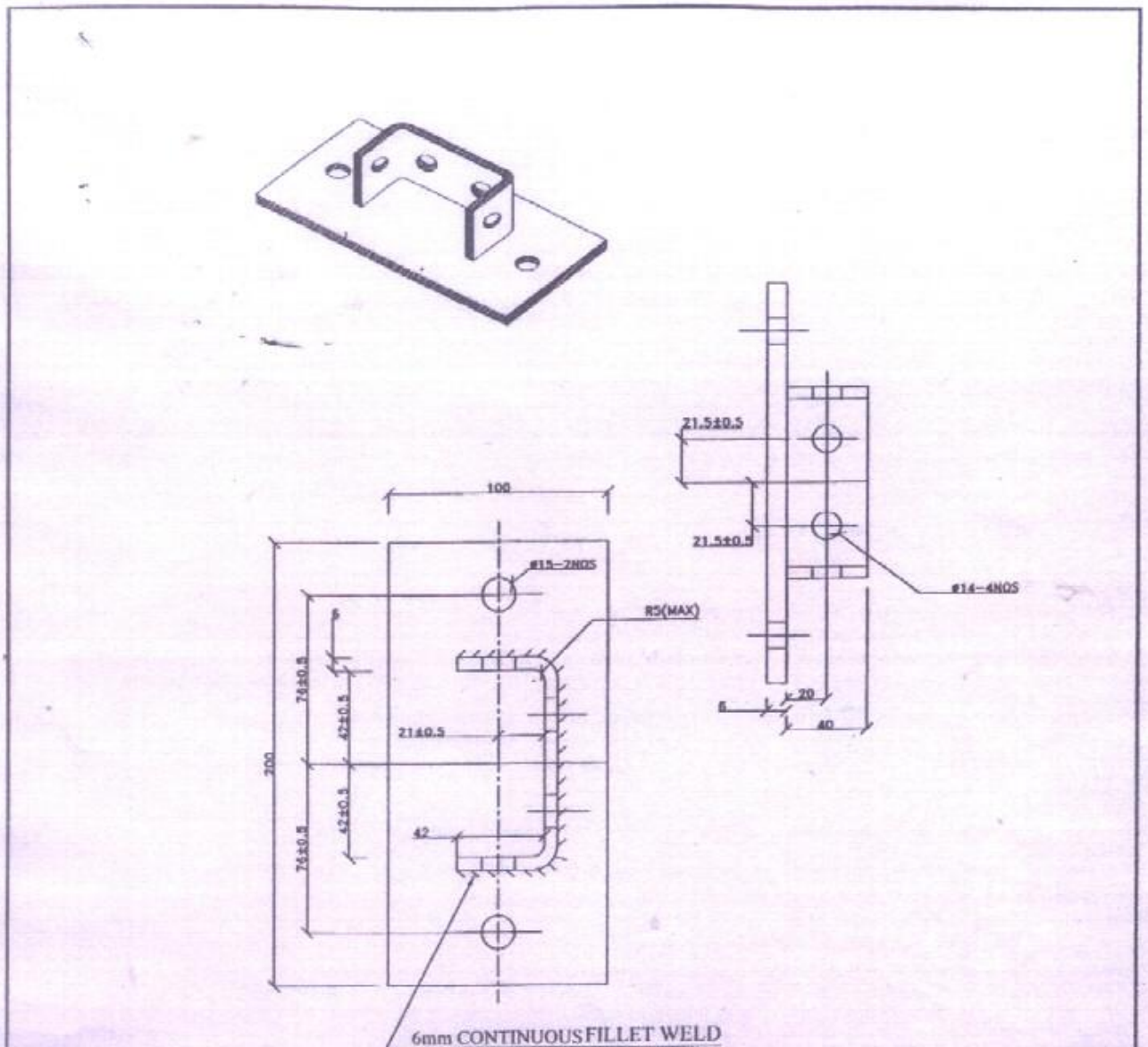
BASE PLATE FOR DOUBLE CHANNEL BP2
