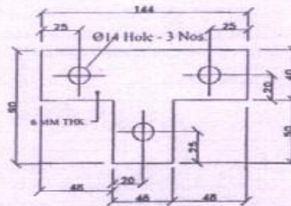
FLAT PLATE TEE FITTING PF1
