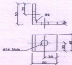
90° ANGLE FITTING LA1
