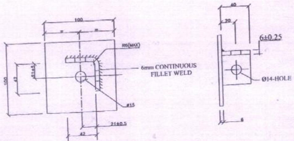
BASE PLATE FOR SINGLE CHANNEL BP1
