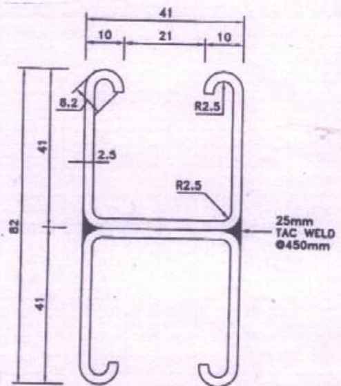
DOUBLE CHANNEL DC1
