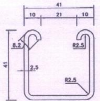
SINGLE CHANNEL SC1
