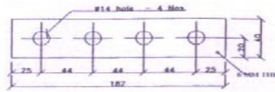
FLAT PLATE STRAIGHT FITTING PF2
