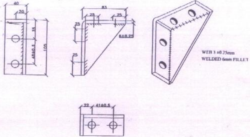
90° ANGLE FITTING H/L
